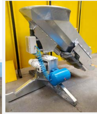
Bottom drive new distribution system with pneumatically activated flap
