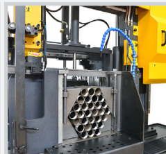
Hexagonal Vice
